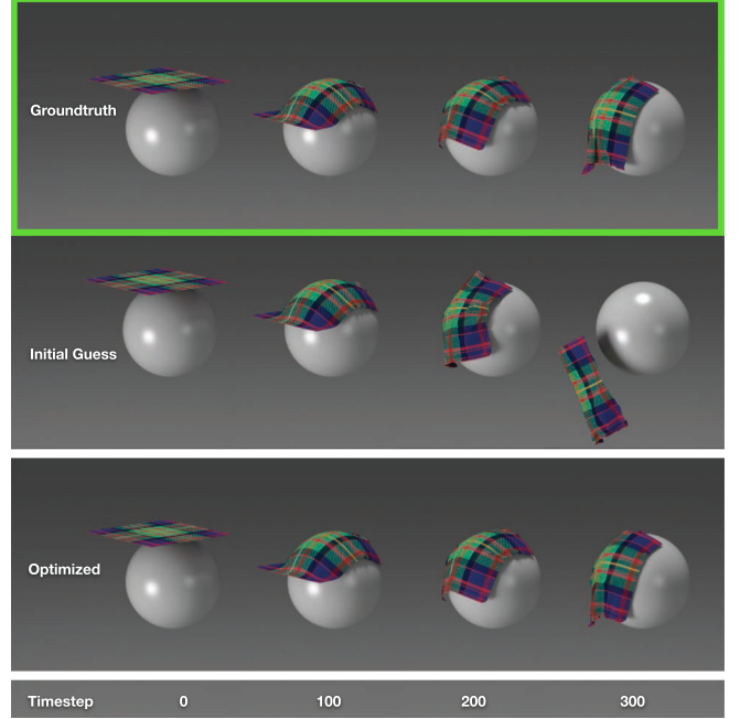
Fig. 8. Sphere (1875 DoFs, h = 1/180s , 350 time steps). Estimating the frictional coefficient \mu between the sphere and the cloth based on the cloth’s contact with the sphere. From top to bottom, we show the simulation at 0, 100, 200, and 300 time steps. Top: the ground-truth motion sequence; Middle: simulation with the initial guess on \mu ; Bottom: simulation after optimization with L-BFGS-B.
