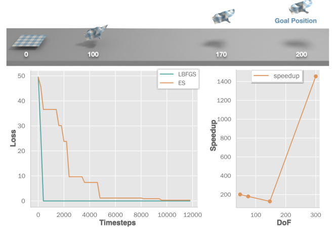
Fig. 4. Flying Napkin. Comparisons between gradient-based and gradient-free methods for optimizing high-dimensional decision variables in differentiable cloth simulation. Top: the motion sequence of a piece of cloth with external forces parametrized with 300 variables. The goal is to find proper external forces with which the cloth ends at a target position. The loss function is defined as the position discrepancy between the simulated motion sequence and the reference motion. Bottom left: the loss vs. time step curves (300 DoF) from gradient-based (L-BFGS-B) and gradient-free (CMA-ES) methods. Both L-BFGS-B and CMA-ES use the same random seeds. Bottom right: we vary the degrees of freedom in the external force parametrization and repeat the experiment three times. For each experiment, we compute the ratio between the number of time steps used by gradient-free and gradient-based methods until they converge or use up the time budget and plot them as a speedup vs. DoFs curve.
